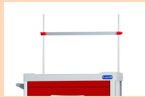
Metal frame with hook 685 L x 26 H x 10 Thickness mm
